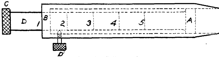
FIG. 1. Soil Sampler.
